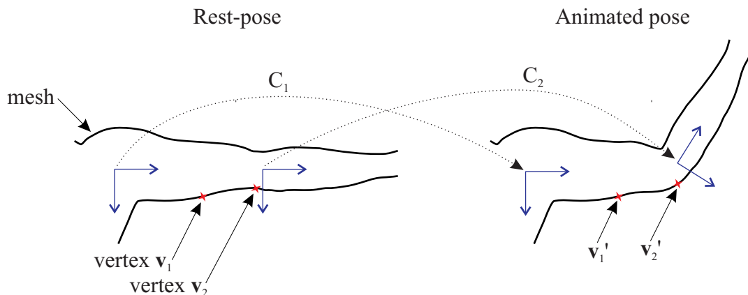
Figure 2.4: A silhouette of human arm animated by matrix palette skinning.
