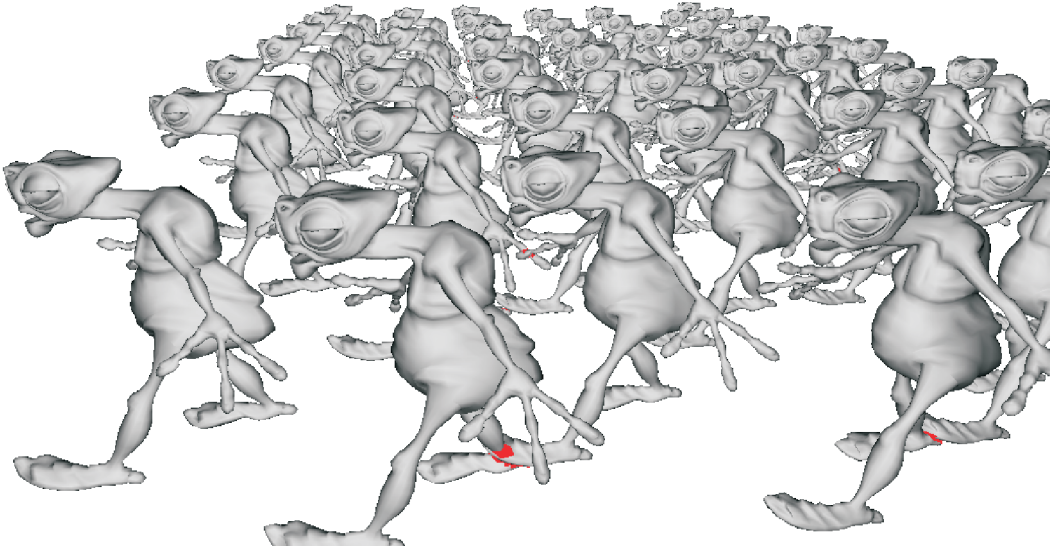
Figure 5.7: The scenario for our crowd collision detection experiment: 50 animated creatures with more than 650 thousands triangles together. Our CD algorithm needs an average 52.83ms per frame, whereas the CD based on complete BVH refitting takes 779.3ms (15-times more).
