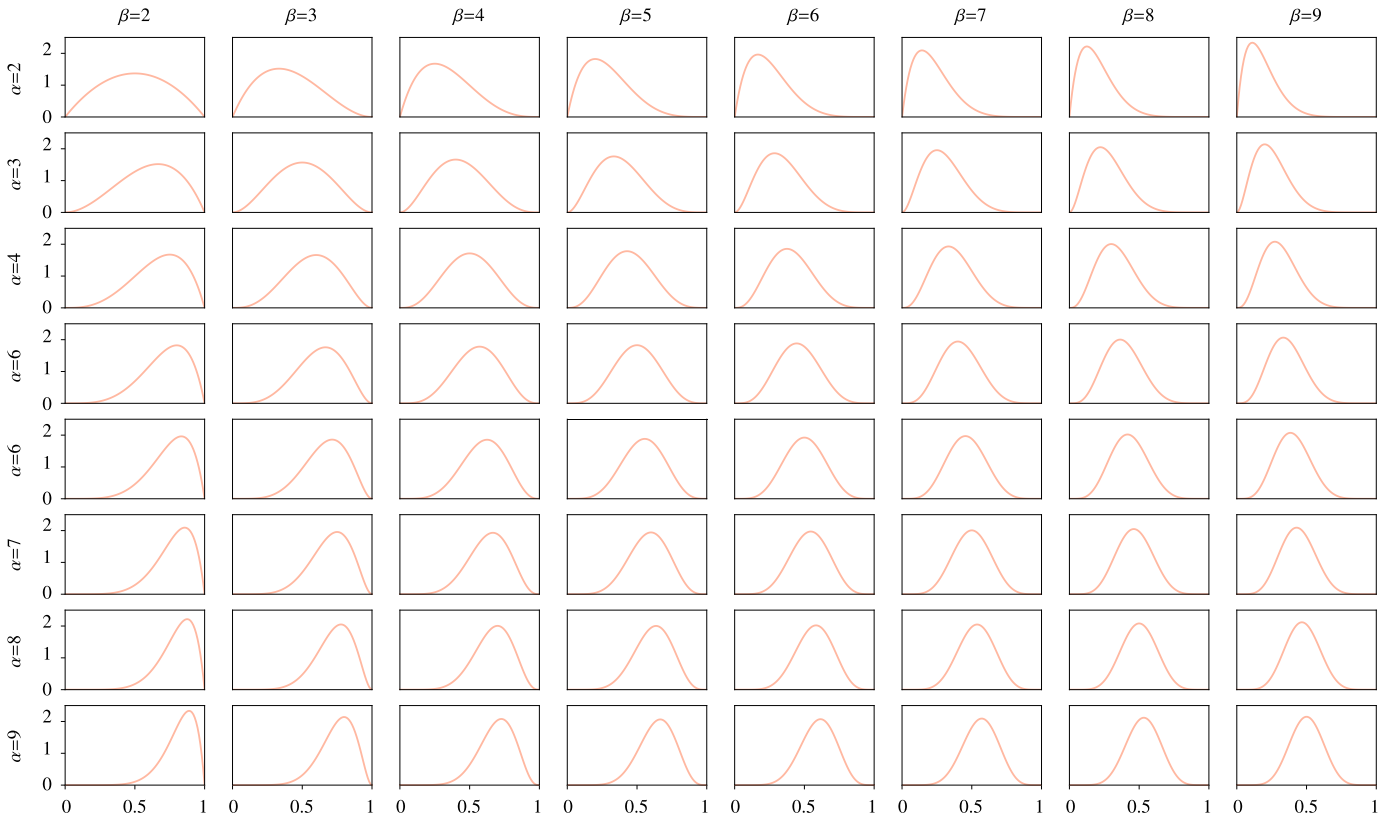
Fig. A1. Profiles of the \varphi function for values of \alpha and \beta .
