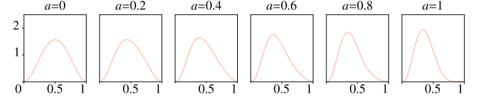
Fig. 6. Profiles of the \Phi function for \alpha_0 = \beta_0 = 3 and (\alpha_1, \beta_1) = (4, 7) .
