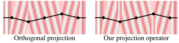
Fig. 4. Comparison between standard point-to-segment orthogonal projection, and ours. Colors are computed w.r.t. the curvilinear axis s(\text{proj}(\mathbf{q})) . Note the discontinuities appearing when using standard orthogonal projection.
