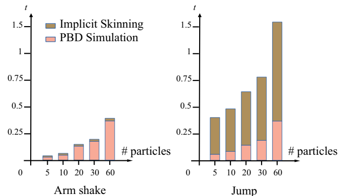
Fig. 12. Average times in seconds for the computation of an animation frame, for different numbers of particles per muscle. The brown represents the computation of Implicit Skinning excluding the PBD simulation, and the pink represents the PBD simulation. (For interpretation of the references to color in this figure legend, the reader is referred to the web version of this article.)
