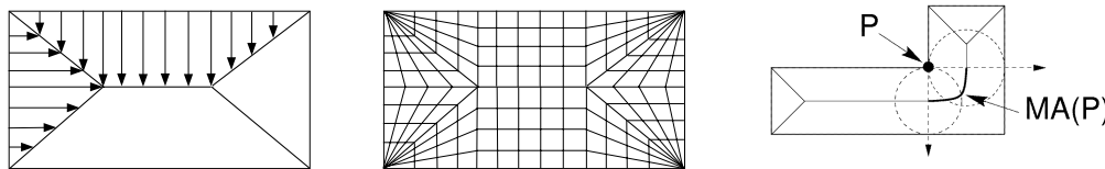
Fig. 4. Weaknesses in a direct medial mapping.
