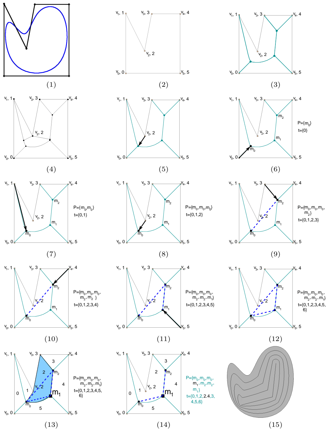
Fig. 8. The concentric completion algorithm, illustrated.
