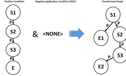
Fig. 7. Pressure Reducing Exam Split Transform.
