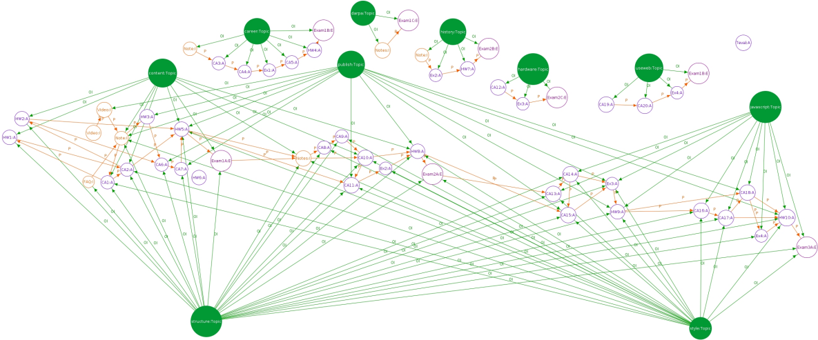
Fig. 11. Course Graph Arranging Learning Items with Clustering by Units.
