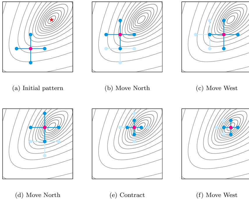
Fig. 1.1 Compass search applied to the modified Broyden tridiagonal function.
