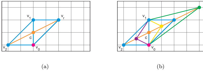
Fig. 4.2 Examples in \mathbb{R}^2 of both (a) the single possible step for the simplex algorithm of Spendley, Hest, and Himsworth and (b) the four basic steps for the Nelder–Mead simplex algorithm.
