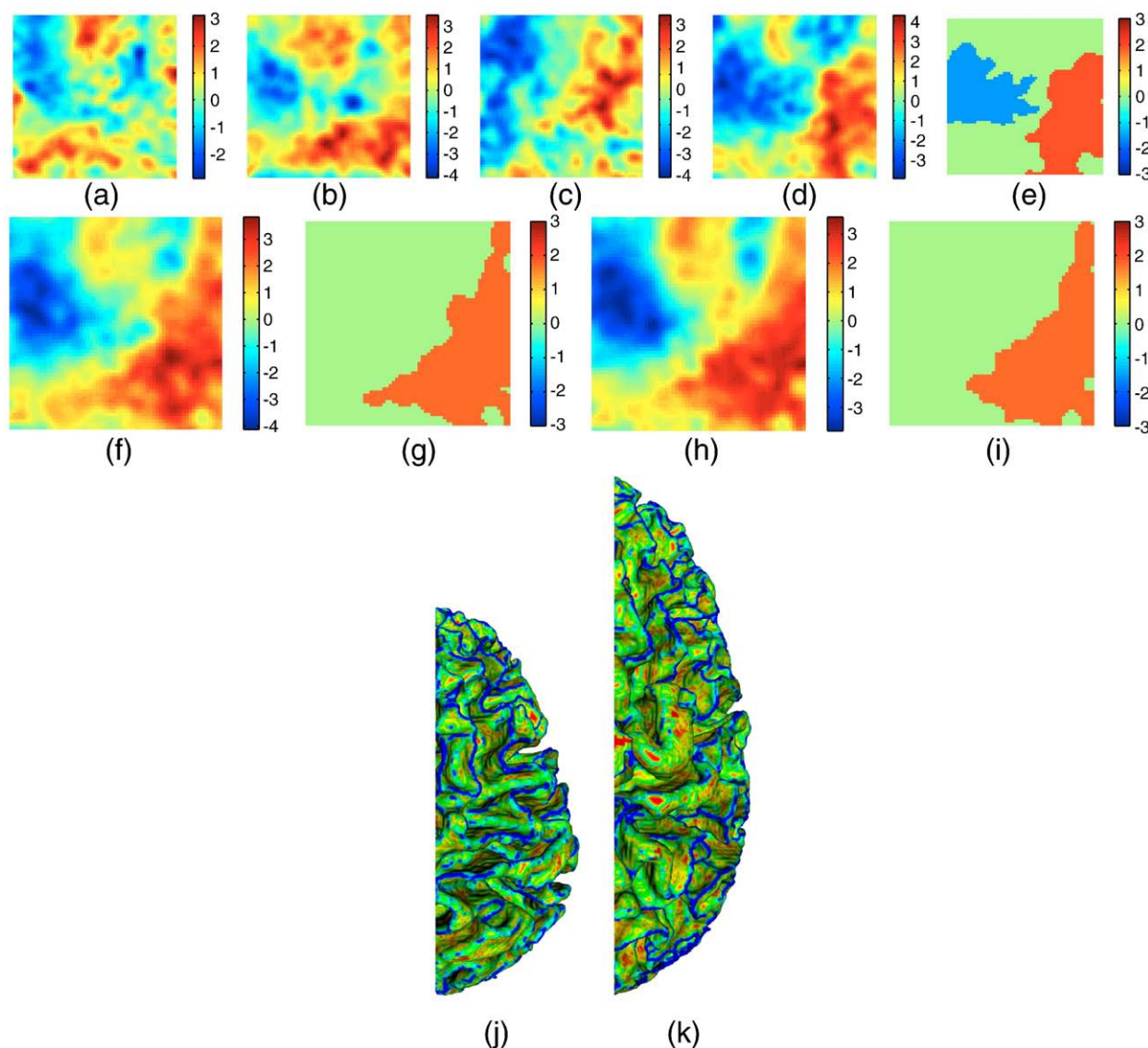
Fig. 5. (a)–(d) Student's t statistics for a cross-sectional study with p^{\text{replication}} (positive t \equiv larger value in males) for frontal, parietal, temporal, and occipital lobes, respectively, in the left hemisphere. Similar patterns exist for lobes in right hemisphere. (e) Significant clusters (via permutation testing) for left occipital lobe. (f), (h) t statistics and (g), (i) significant clusters (via permutation testing) for p^{\text{replication}} for left hemisphere (4 lobes) and whole brain (8 lobes), respectively. A similar pattern exists for the right hemisphere. Note the larger mass (red) for males in the low-curvedness regions (bottom half) and larger mass (red) for males in the convex regions (right half). (j)–(k) Selected smaller-than-average female and larger-than-average male brains, respectively, painted by C values (red \rightarrow blue \equiv zero \rightarrow high) to enable/accentuate visualization of the differences. Thus, based on the meaning of complexity ingrained in p^{\text{replication}} , the female cortex appears more “complex”, i.e. more blue/cyan. Compare this with Fig. 6(e–f). (For interpretation of the references to colour in this figure legend, the reader is referred to the web version of this article.)
