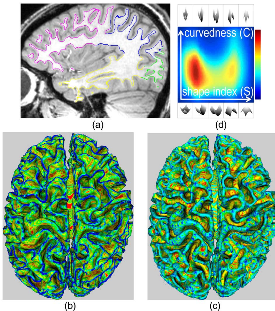
Fig. 1. (a) A sagittal slice of a head MR image overlapped with the cortical surface \mathcal{M} . (b) Curvedness values C(m) painted on \mathcal{M} (red \rightarrow blue \equiv zero \rightarrow high). In this figure, red areas are almost flat and blue areas are highly curved. (c) Shape index values S(m) \in [-1, 1] painted on \mathcal{M} (red \rightarrow blue \equiv -1 \rightarrow 1 ). In this figure, red/yellow areas are concave, blue/cyan areas are convex, and green areas are saddles. (d) Proposed descriptor P_{\mathcal{M}}(C, S) (blue \rightarrow red \equiv 0 \rightarrow 1 probability; colormap shown on right). For all plots of P_{\mathcal{M}}(C, S) in this paper: horizontal axis \equiv S , vertical axis \equiv C . The illustrations of local surface patches, at the top and bottom of this figure, depict patches for the entire range of possible S values; corresponding patches at the top and bottom have the same S value; all patches at the top have the same C value that is higher than the C value for all the patches at the bottom; the left half of the domain comprises concave patches, while the right half comprises convex patches. (For interpretation of the references to colour in this figure legend, the reader is referred to the web version of this article.)
