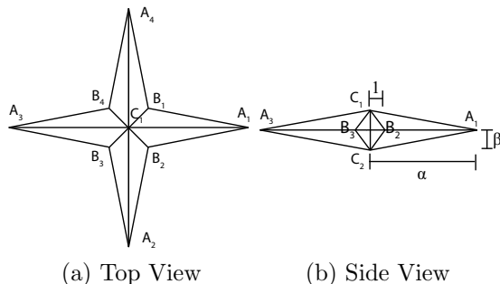
Figure 1: Polyhedron P_4(\alpha, \beta)
