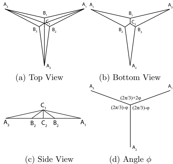
Figure 2: The polyhedron P_3^\phi(\alpha, \beta)
