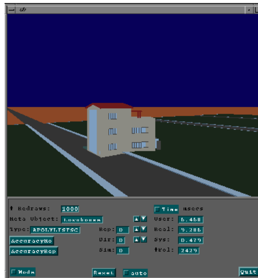
Figure C: Measuring the rendering cost of a representation.
