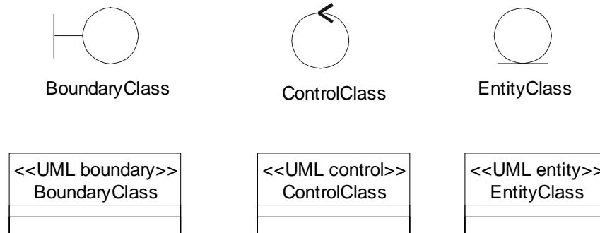
Figure 2.6 Objectory Process Classes, With and Without Stereotype Icons
