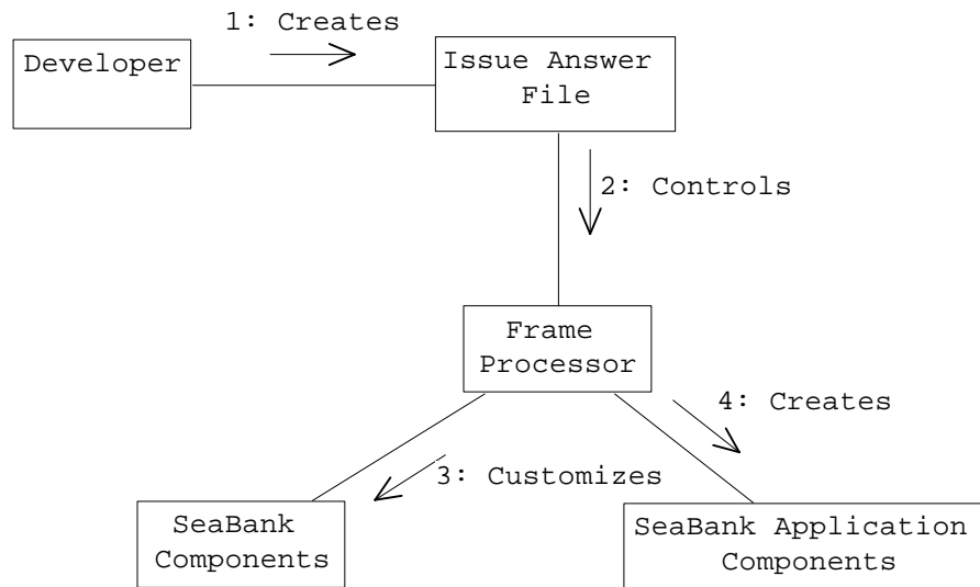
Figure 3.1 SeaBank Manual Component Development Process
