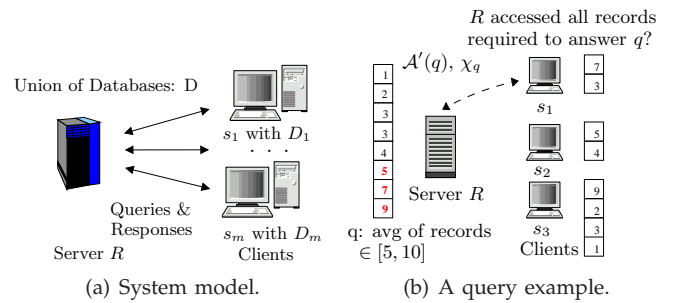
Fig. 1. Query access assurance in distributed databases.
