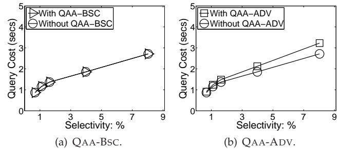
Fig. 6. Server-side query cost vs. \rho_q .
