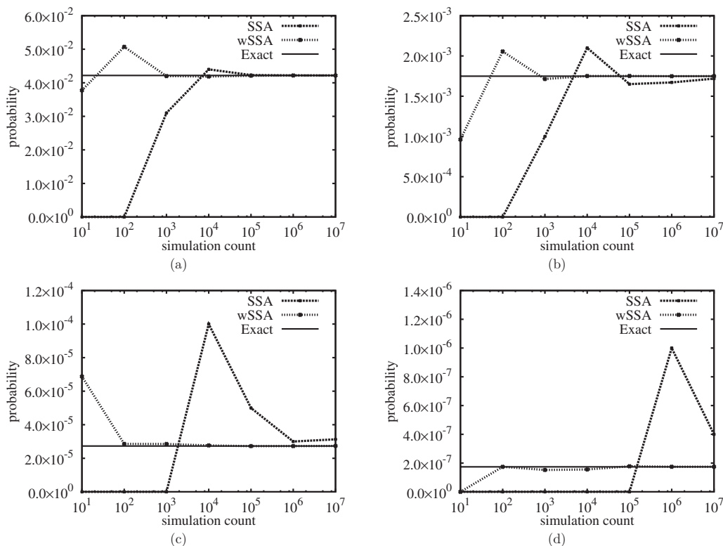
FIG. 4. Changes of the estimated P_{t \leq 100}(X_5 \rightarrow \theta | \mathbf{x}_0) via the SSA and the wSSA with respect to simulation counts for each \theta . The solid line represents the true probability. (a) \theta=40 , (b) \theta=35 , (c) \theta=30 , and (d) \theta=25 .
