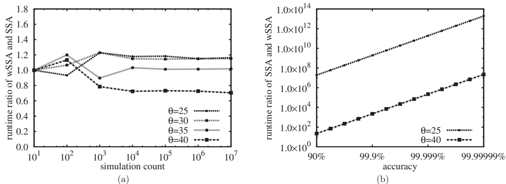
FIG. 6. Comparison of runtime between the SSA and the wSSA for the simulation of reaction (16). (a) The ratio of the simulation time of the wSSA and the SSA with respect to simulation counts for the four values of \theta . (b) Ratio of the computational time between the SSA and the wSSA with respect to a given level of accuracy \epsilon .
