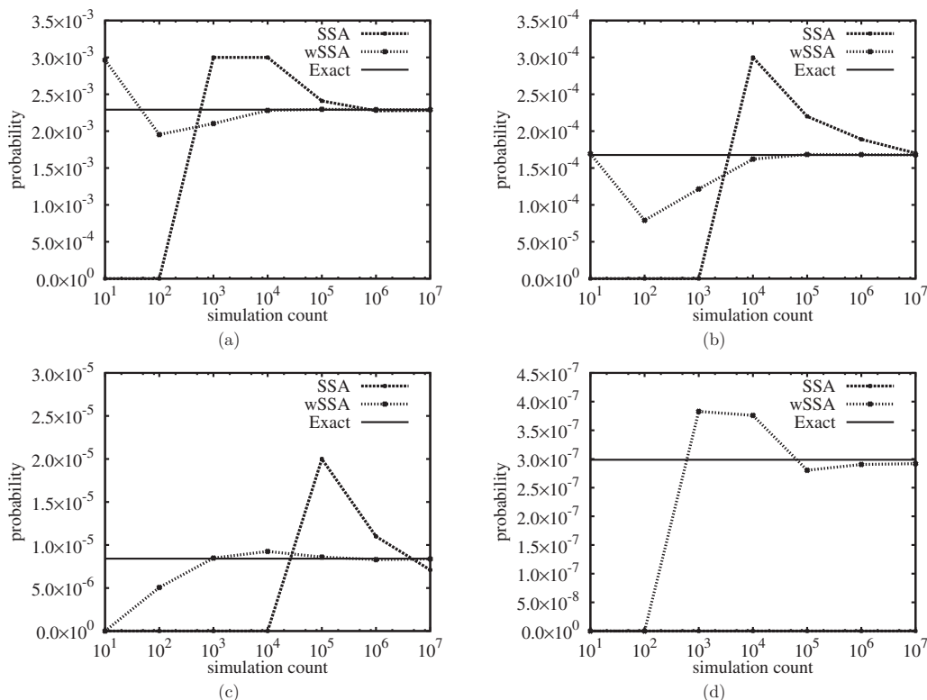
FIG. 1. Changes of the estimated P_{t \leq 100}(X_2 \rightarrow \theta | \mathbf{x}_0) via the SSA and the wSSA with respect to simulation counts for each \theta . The solid line represents the true probability. (a) \theta=65 , (b) \theta=70 , (c) \theta=75 , and (d) \theta=80 .
