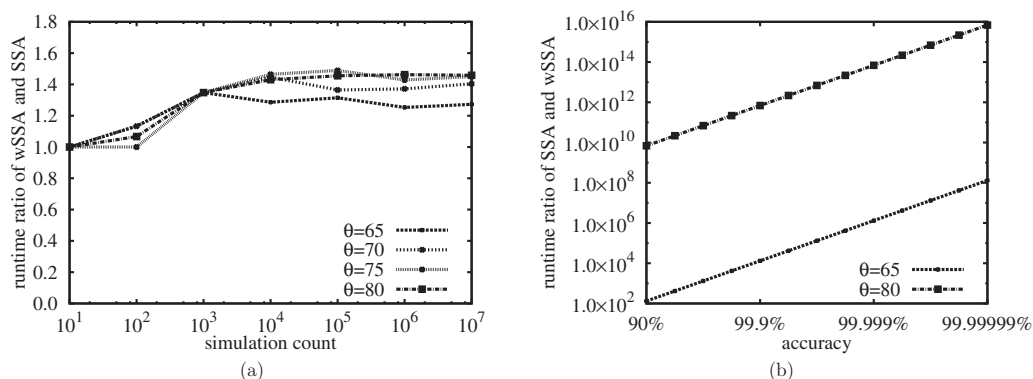
FIG. 3. Comparison of runtime between the SSA and the wSSA for the simulation of reaction (15). (a) Ratio of the simulation time between the wSSA and the SSA with respect to simulation counts for the four values of \theta . (b) Ratio of computational time between the SSA and the wSSA with respect to a given level of accuracy \epsilon .
