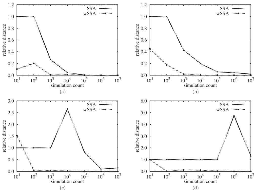
FIG. 5. Changes of the relative distance between the true value and the estimate value of P_{t \leq 100}(X_5 \rightarrow \theta | \mathbf{x}_0) via the SSA and the wSSA with respect to simulation counts for each \theta . (a) \theta=40 , (b) \theta=35 , (c) \theta=30 , and (d) \theta=25 .
