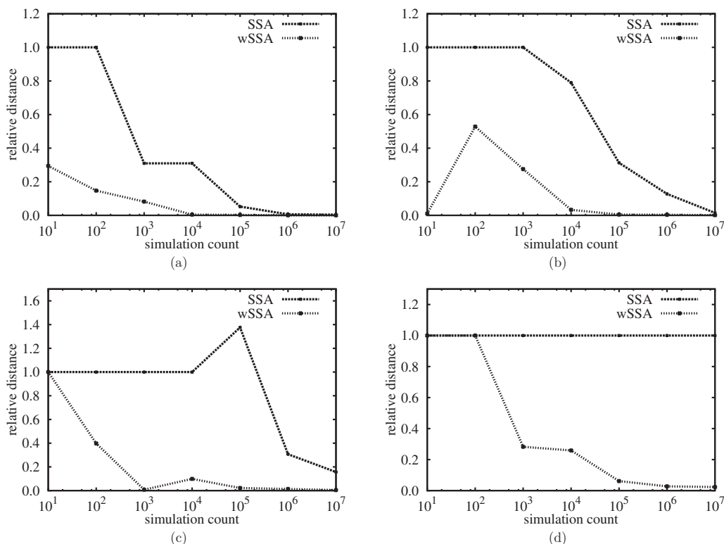
FIG. 2. Changes of the relative distance between the true value and the estimate value of P_{t \leq 100}(X_2 \rightarrow \theta | \mathbf{x}_0) via the SSA and the wSSA with respect to simulation counts for each \theta . (a) \theta=65 , (b) \theta=70 , (c) \theta=75 , and (d) \theta=80 .
