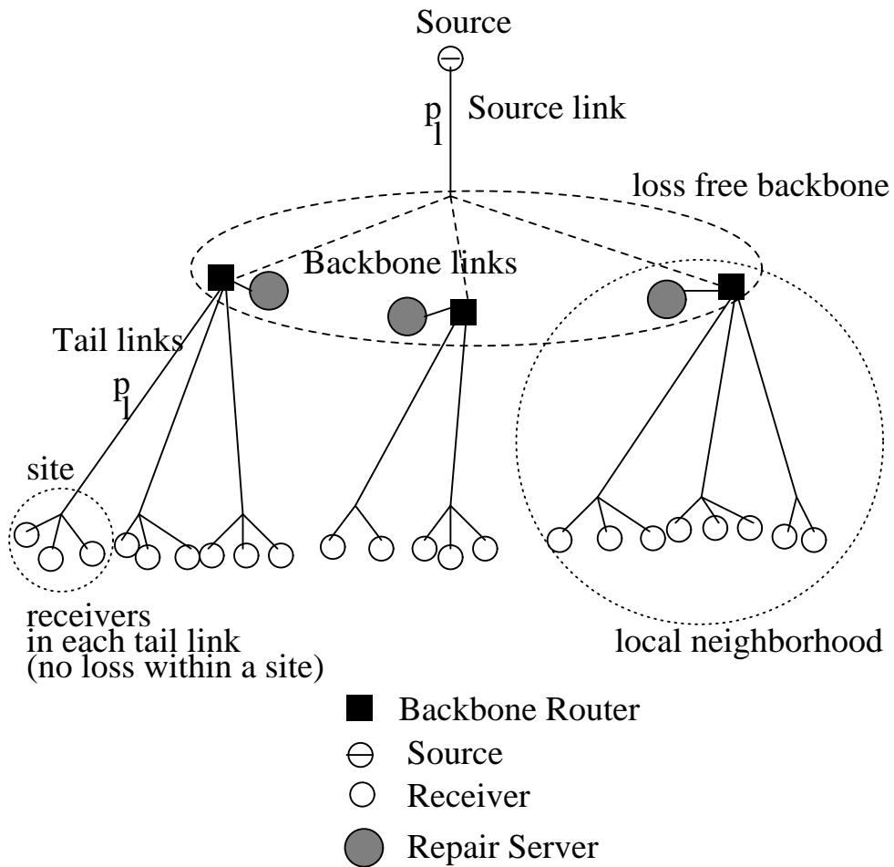
Figure 1: System Model
