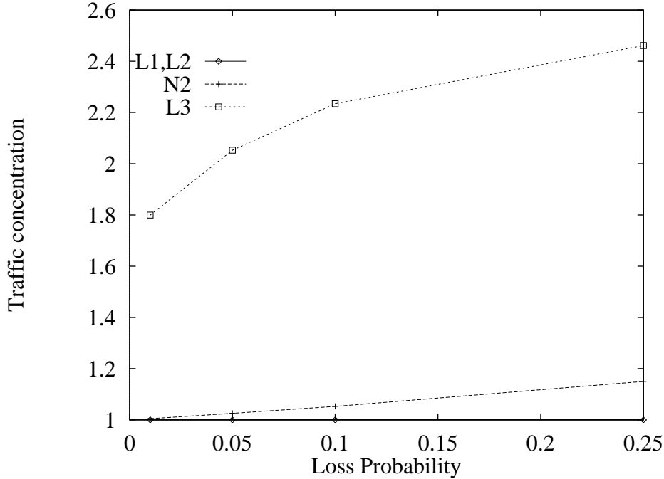
Figure 6: Traffic Concentration
