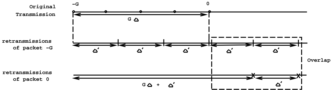
Figure 8: Sender timeline
