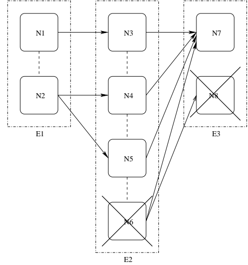
Figure 5: Example of an InSeq Violation
