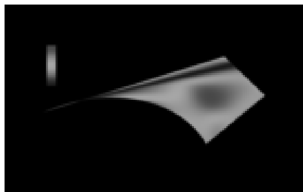
Twist component of a nonplanar twisted surface.
