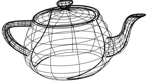
Figure 1: Silhouettes are equivalent to the zero set of equation 6 (rotated view).
