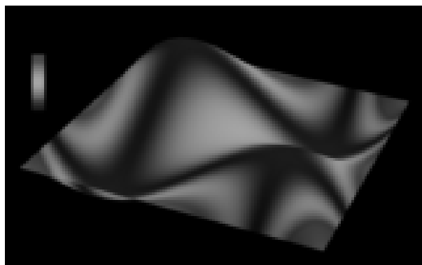
Twist component of a surface (same surface as in plate 2).
