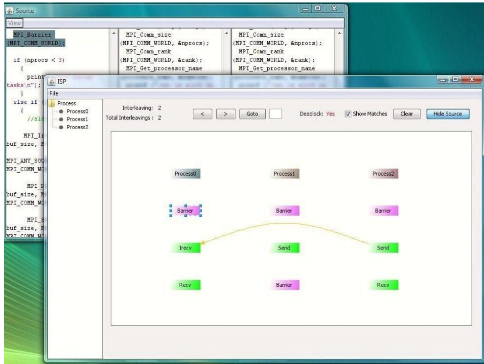
Figure 2: Screenshot of ispUI - showing deadlocking interleaving for the example any_src-can-deadlock9.c
