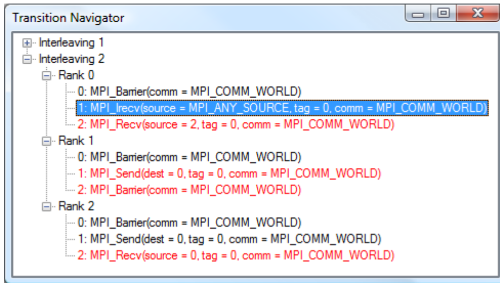
Figure 7: Visual Studio transition Navigator
