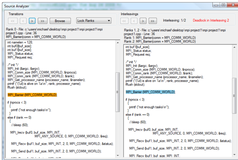
Figure 5: ISP Source Analyzer
