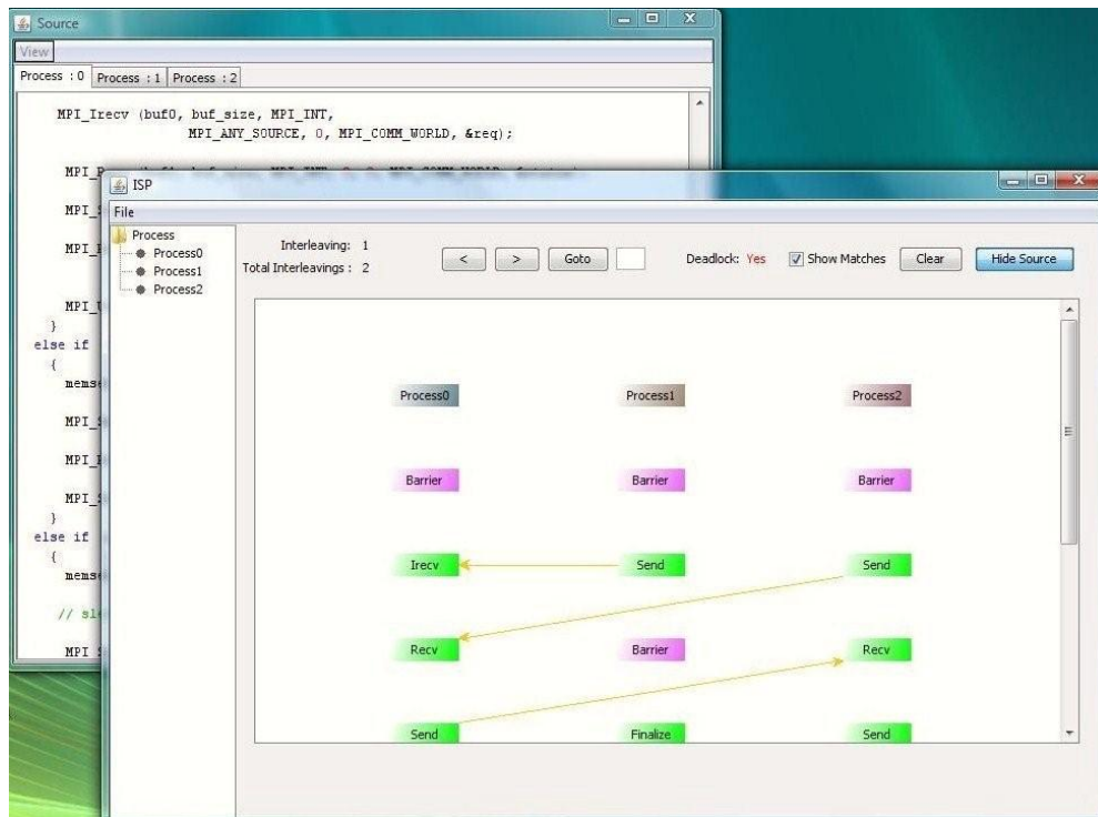
Figure 1: Screenshot of ispUI - showing non-deadlocking interleaving for the example any_src-can-deadlock9.c
