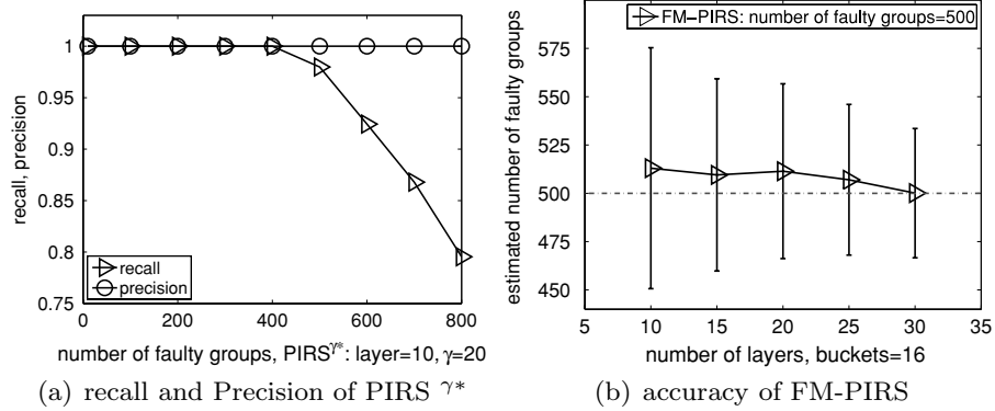
Fig. 8. Effectiveness of PIRS \gamma^* and FM-PIRS.
