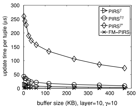
Fig. 6. Space-time trade-off.
